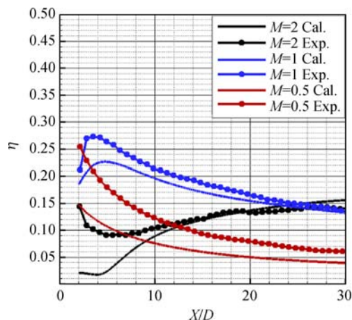
图9 冷却效率展向平均分布实验结果和计算结果对比 Fig. 9 Comparison of laterally averaged cooling effectiveness distribution between experiment result and calculation result
