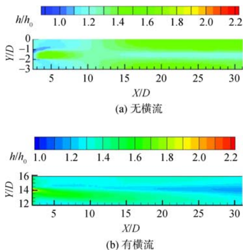
图8 M=2时有无横流表面传热系数对比 Fig. 8 Comparison of heat transfer coefficient with and without crossflow for M=2
