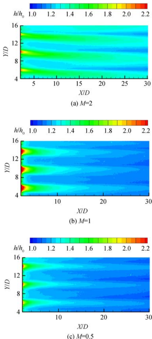
图7 横流条件下不同吹风比表面传热系数云图 Fig. 7 Contours of heat transfer coefficient with crossflow under different blowing ratios
